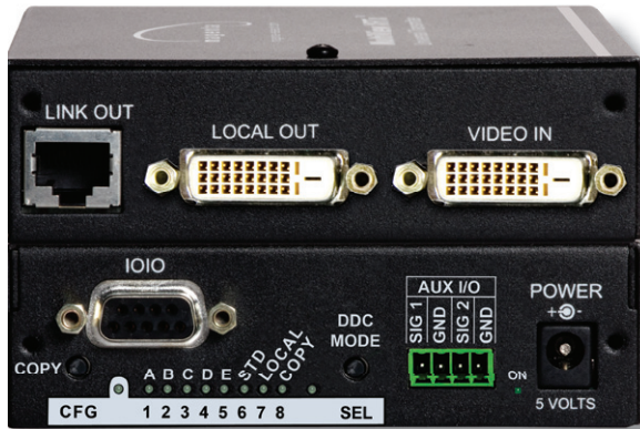
MULTIVIEW DVI TRANSMITTER FRONT/BACK VIEW (-SAP VERSION)
