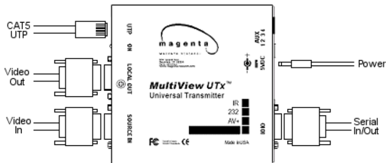
Figure 3-3. Connections on the UTx 232 Universal Transmitter.
